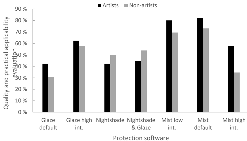
Figure 10. Assessment of the quality and practical applicability of protected images.
